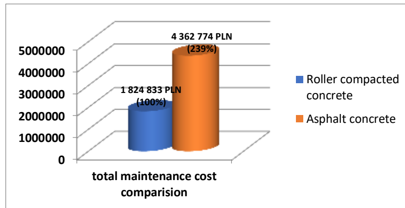
Figure 6. Comparison of the total maintenance cost.
